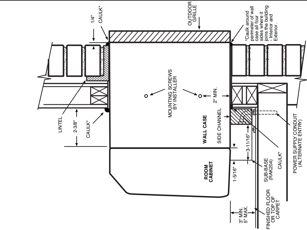
Sub-Base Connected
